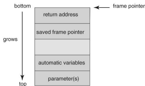
Figure- The layout for a typical stack frame.
