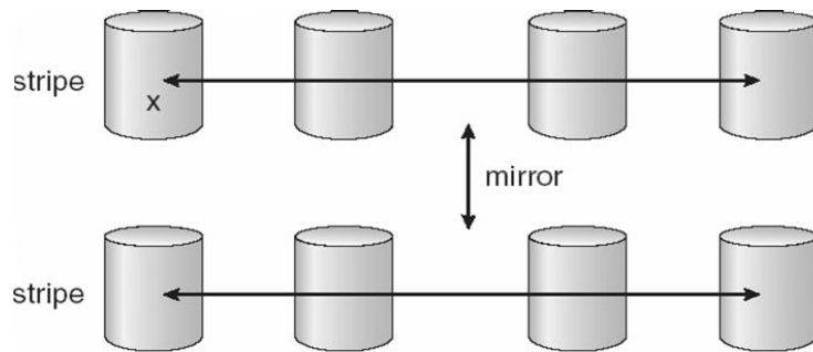
a) RAID 0 + 1 with a single disk failure.
